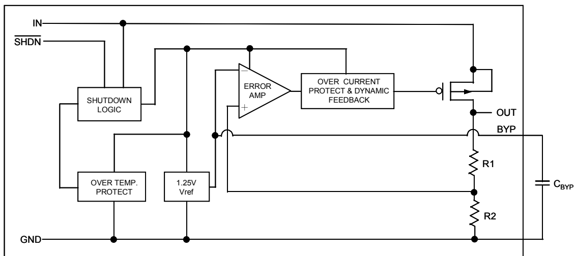
Figure 1. Functional Diagram
