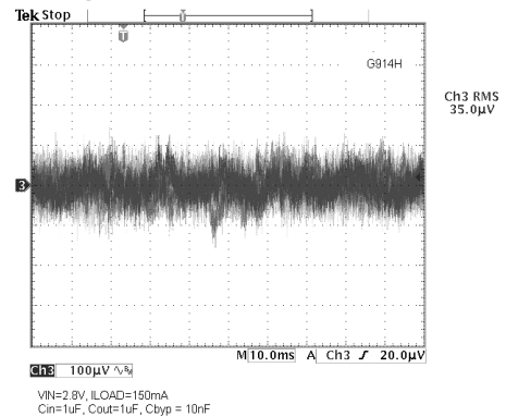
Output Noise 10KHZ to 100KHZ
