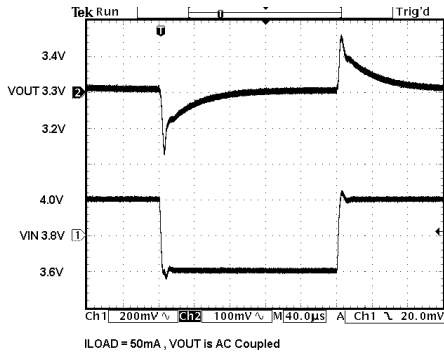
Line Transient
