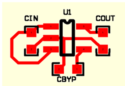
Figure 4. Fixed Mode
