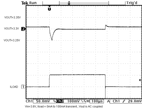
Load Transient
