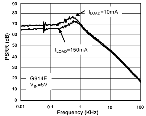
Power Supply Rejection Ripple
