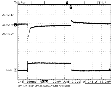
Load Transient
