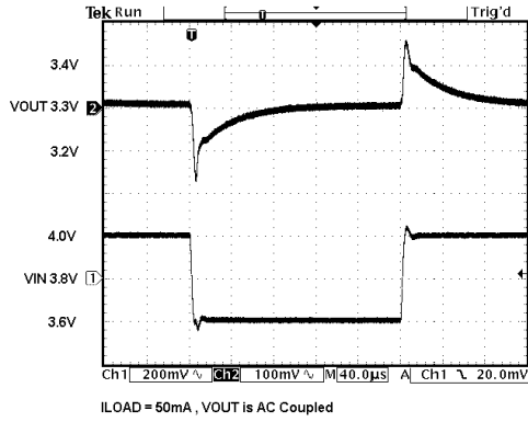
Line Transient
