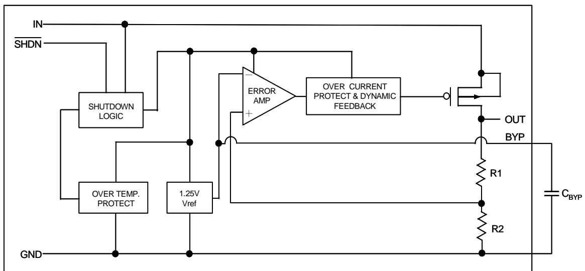
Figure 1. Functional Diagram
