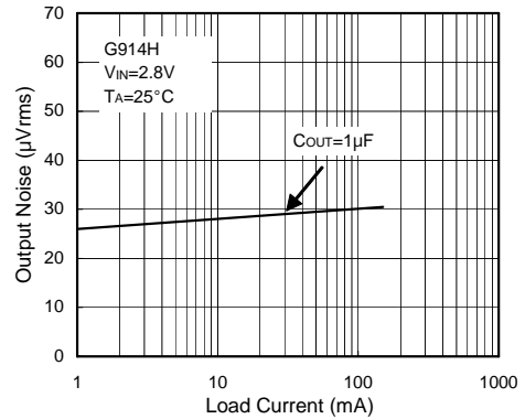
Output Noise vs. Load Current
