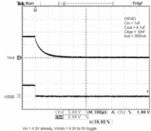
Shutdown Delay Waveform
