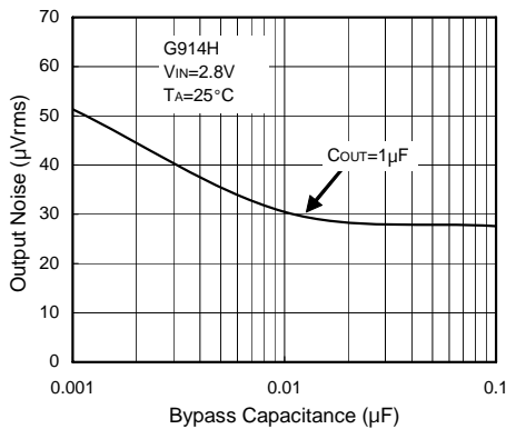
Output Noise vs. Bypass Capacitance
