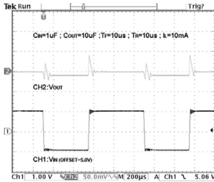
Line Transient
