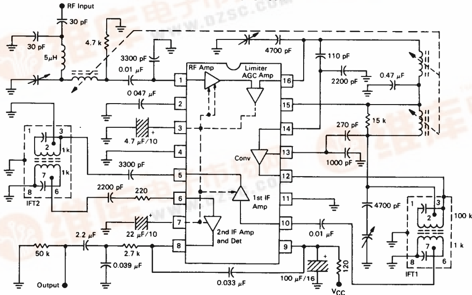
FIGURE 1 — TEST CIRCUIT
