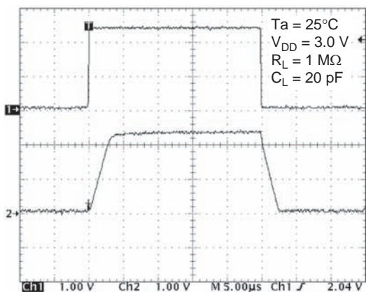
Figure 3-19. HA1630D03 Large Signal Transient Response
