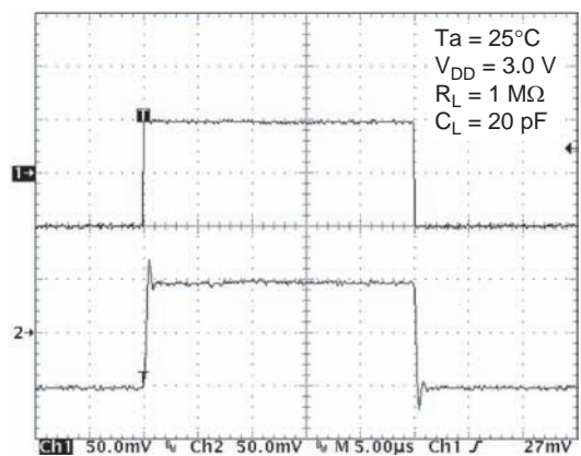
Figure 3-20. HA1630D03 Small Signal Transient Response
