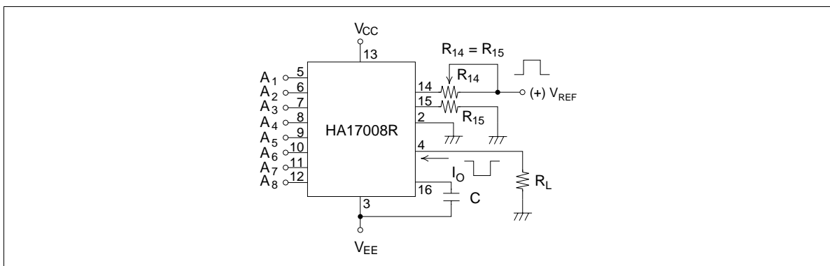
Figure 1 Positive Reference Potential Application Example
