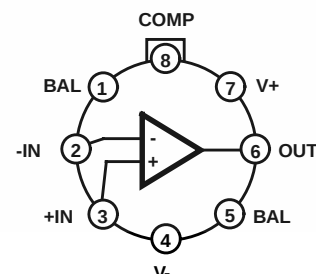
HA-2620, HA-2625 (METAL CAN) TOP VIEW
