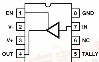
HA4201 (8 LD SOIC) TOP VIEW
