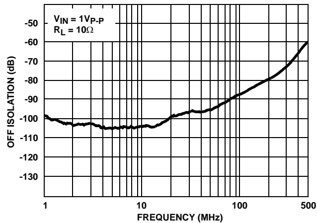
FIGURE 7. OFF ISOLATION
