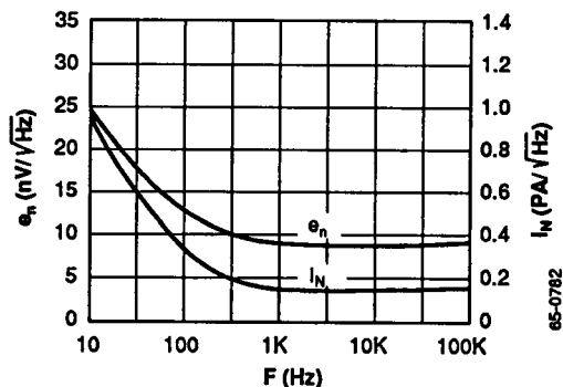
Input Noise Voltage vs. Frequency
