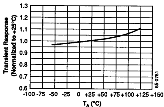
Transient Response vs. Temperature
