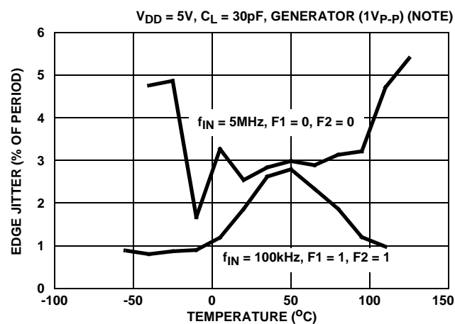
FIGURE 30. EDGE JITTER vs TEMPERATURE
