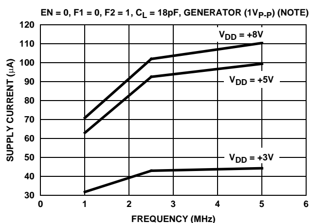
FIGURE 16. DISABLED SUPPLY CURRENT vs FREQUENCY
