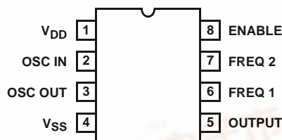
HA7210 (PDIP, SOIC) TOP VIEW
