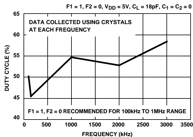
FIGURE 27. DUTY CYCLE vs FREQUENCY
