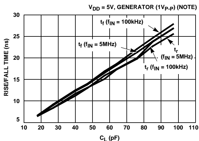
FIGURE 33. RISE/FALL TIME vs C_L
