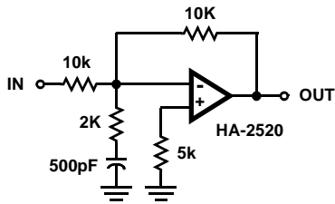
FIGURE 6. INVERTING UNITY GAIN CIRCUIT
