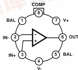
HA-2520, HA-2522, HA-2525 (8 LD METAL CAN) TOP VIEW
