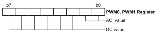
Pulse Width Modulation Registers
