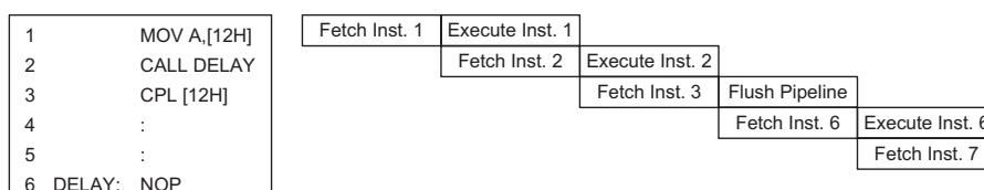
System Clocking and Pipelining
