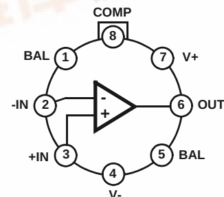
HA-2640/2645 (METAL CAN) TOP VIEW
