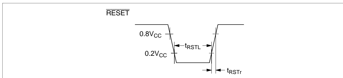
Figure 68 \overline{RESET} Timing
