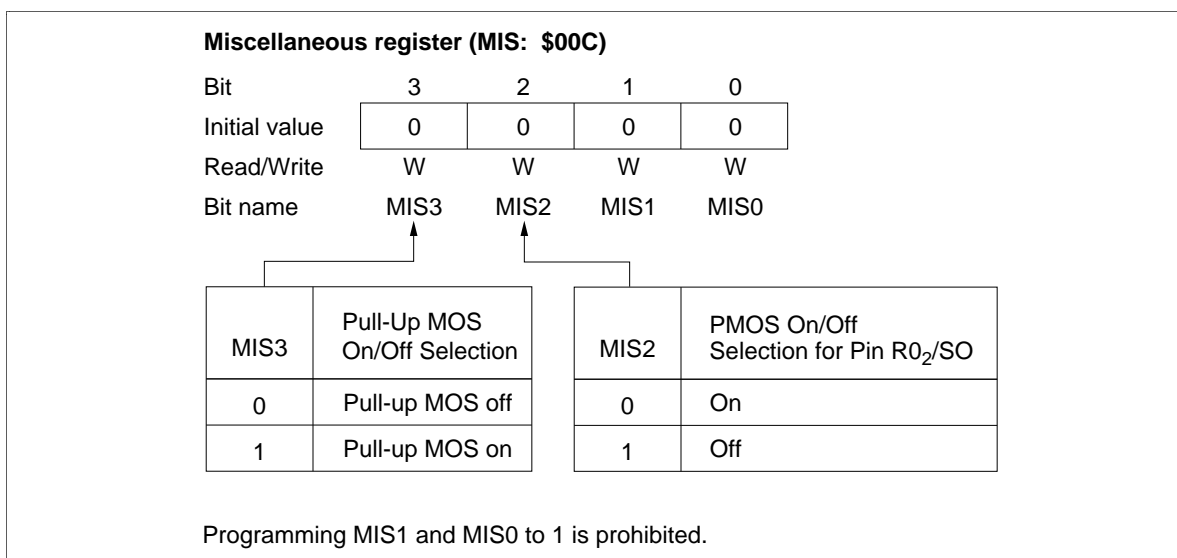
Figure 24 Miscellaneous Register
