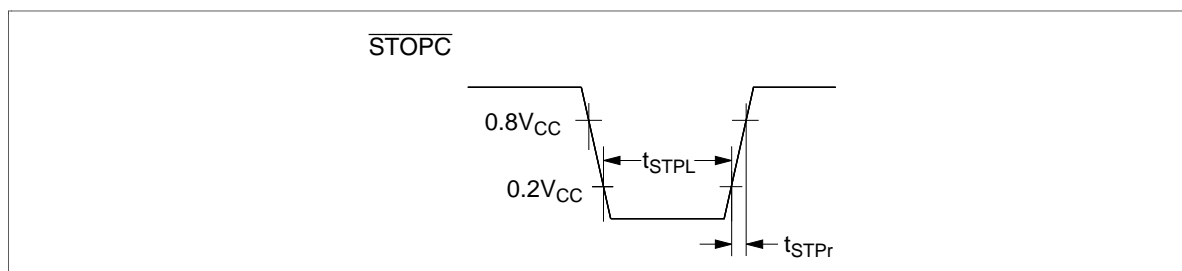
Figure 69 \overline{STOPC} Timing
