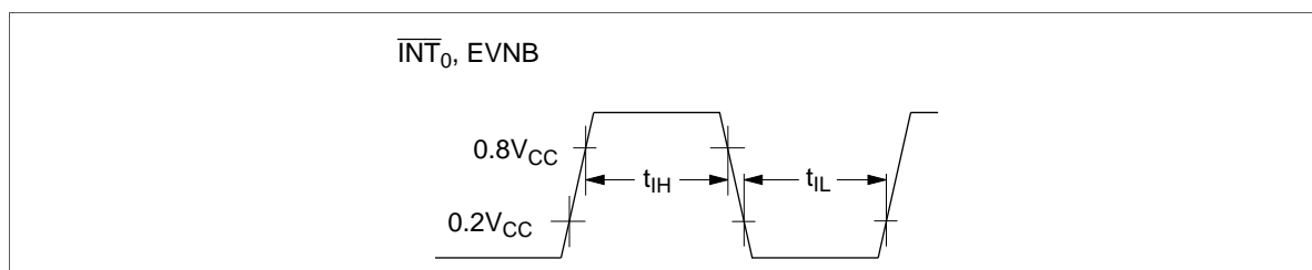
Figure 67 Interrupt Timing
