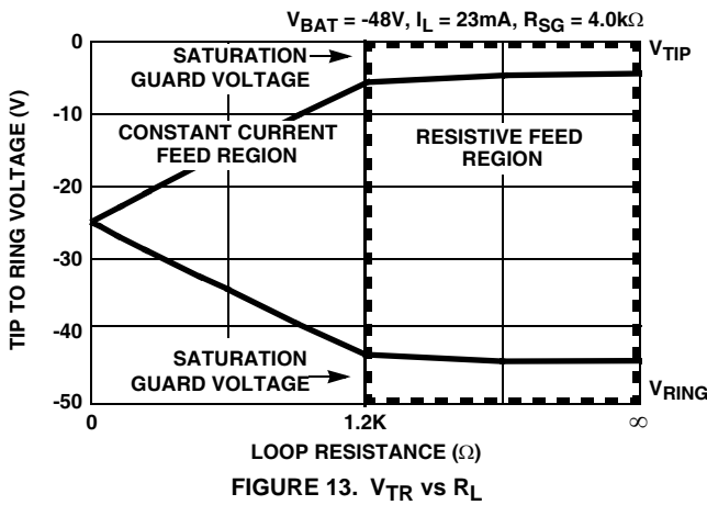
FIGURE 13. V_{TR} vs R_L
