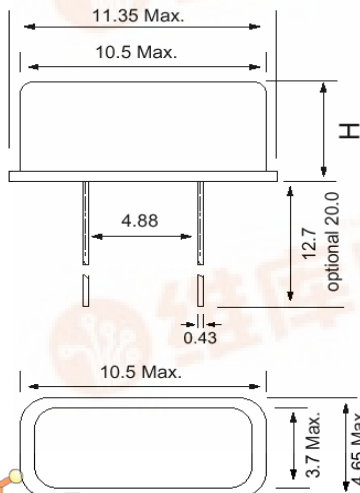
Figure 1) HC-49US-DN - Top and Side Views
