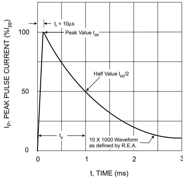
Fig. 3 Pulse Waveform
