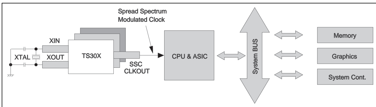
Fig 5 XTAL Ref. Clock Input Example
