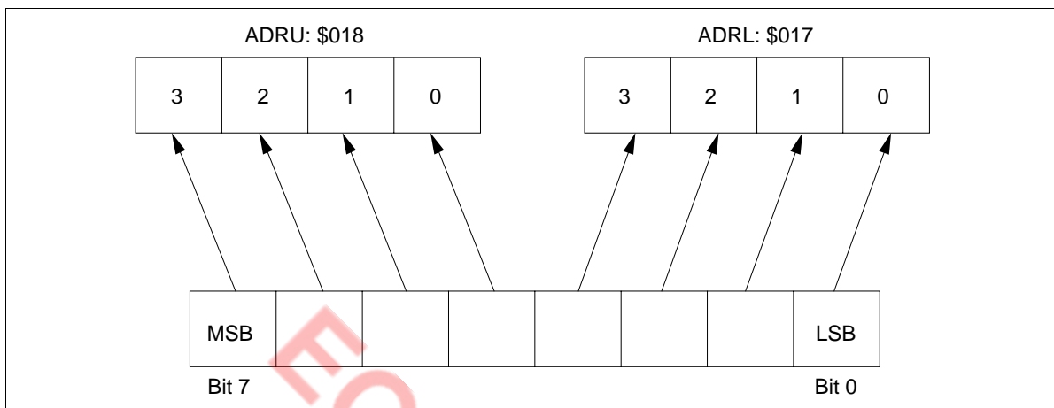
Figure 75 A/D Data Registers (ADRU, ADRL)
