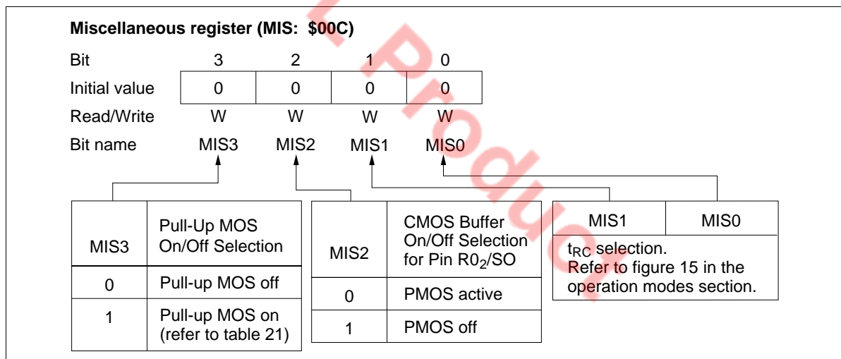
Figure 34 Miscellaneous Register (MIS)
