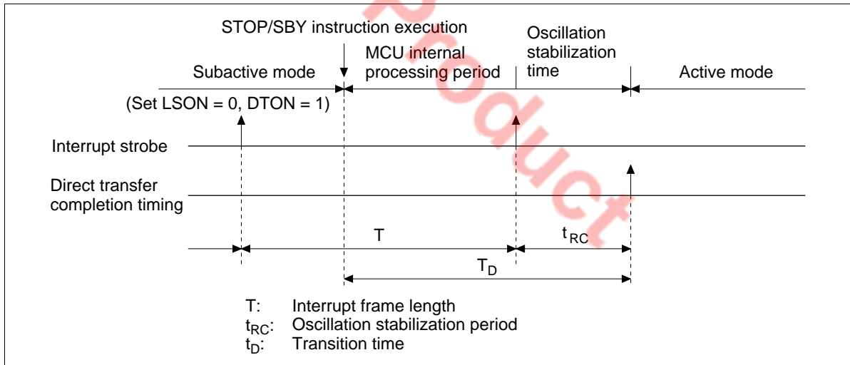
Figure 16 Direct Transition Timing
