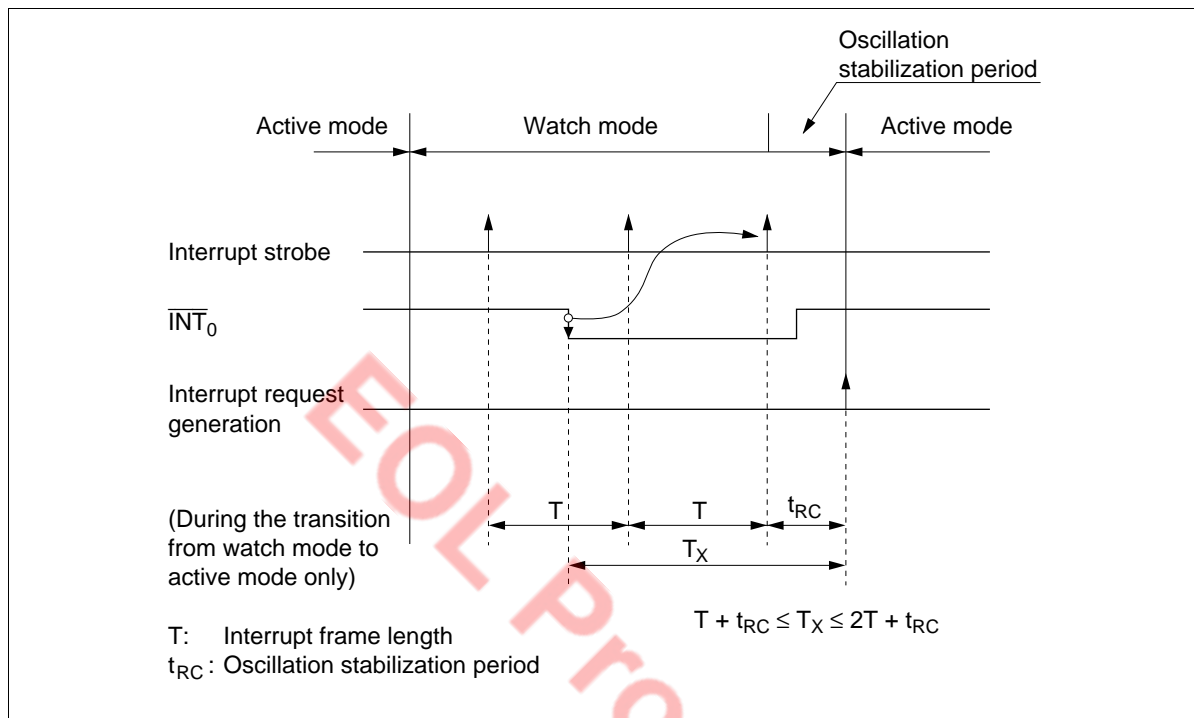
Figure 14 Interrupt Frame
