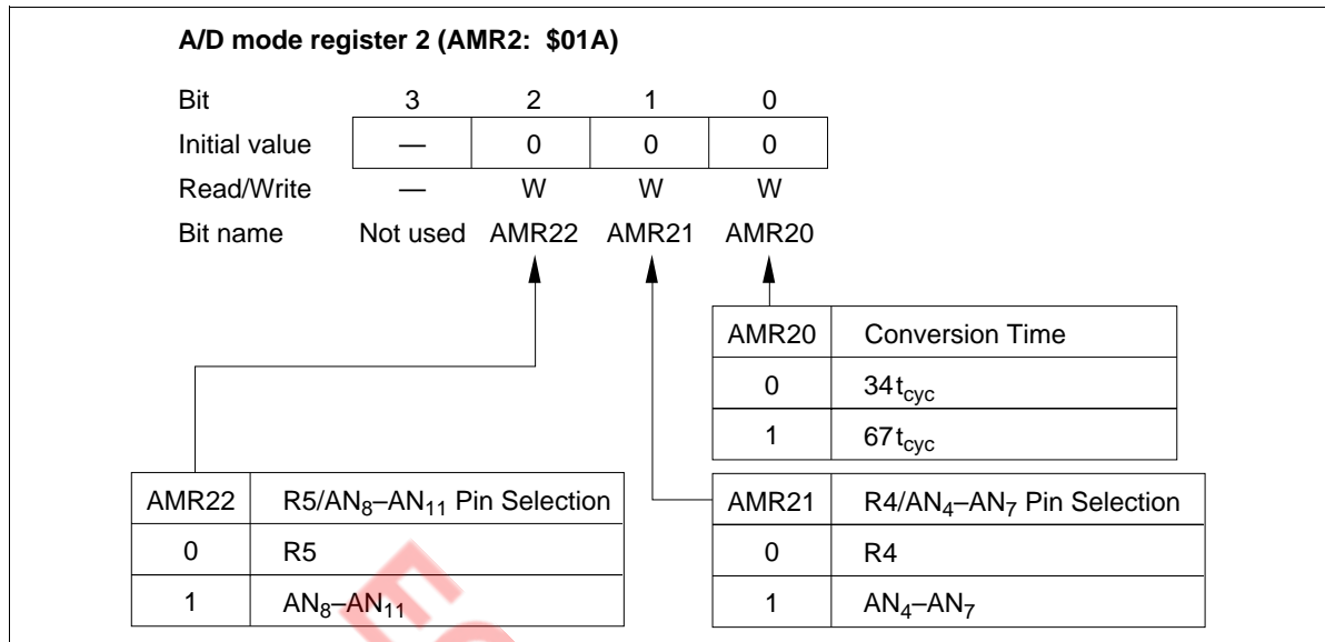
Figure 33 A/D Mode Register 2 (AMR2)
