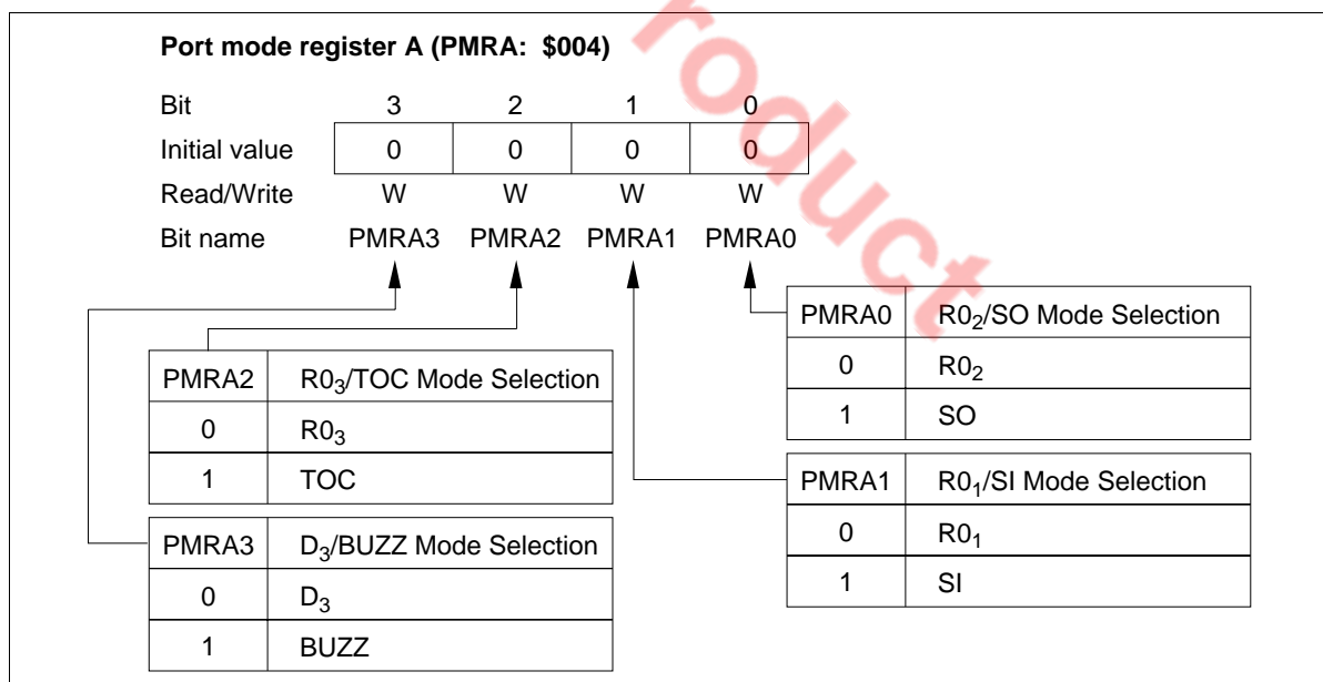
Figure 30 Port Mode Register A (PMRA)
