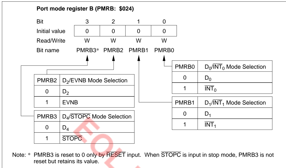
Figure 29 Port Mode Register B (PMRB)
