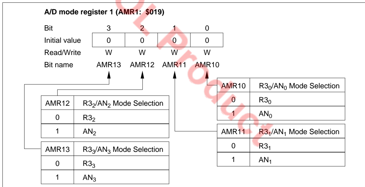
Figure 32 A/D Mode Register 1 (AMR1)
