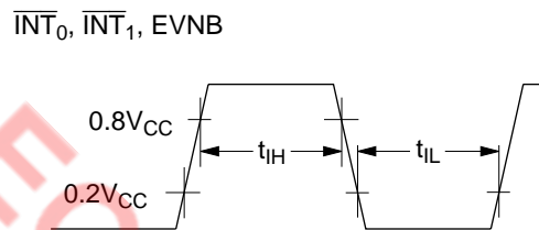
Figure 85 Interrupt Timing
