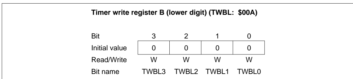
Figure 42 Timer Write Register B Lower Digit (TWBL)
