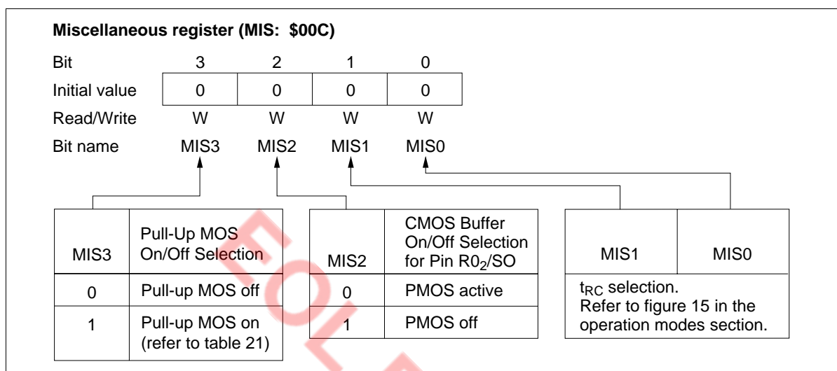
Figure 68 Miscellaneous Register (MIS)
