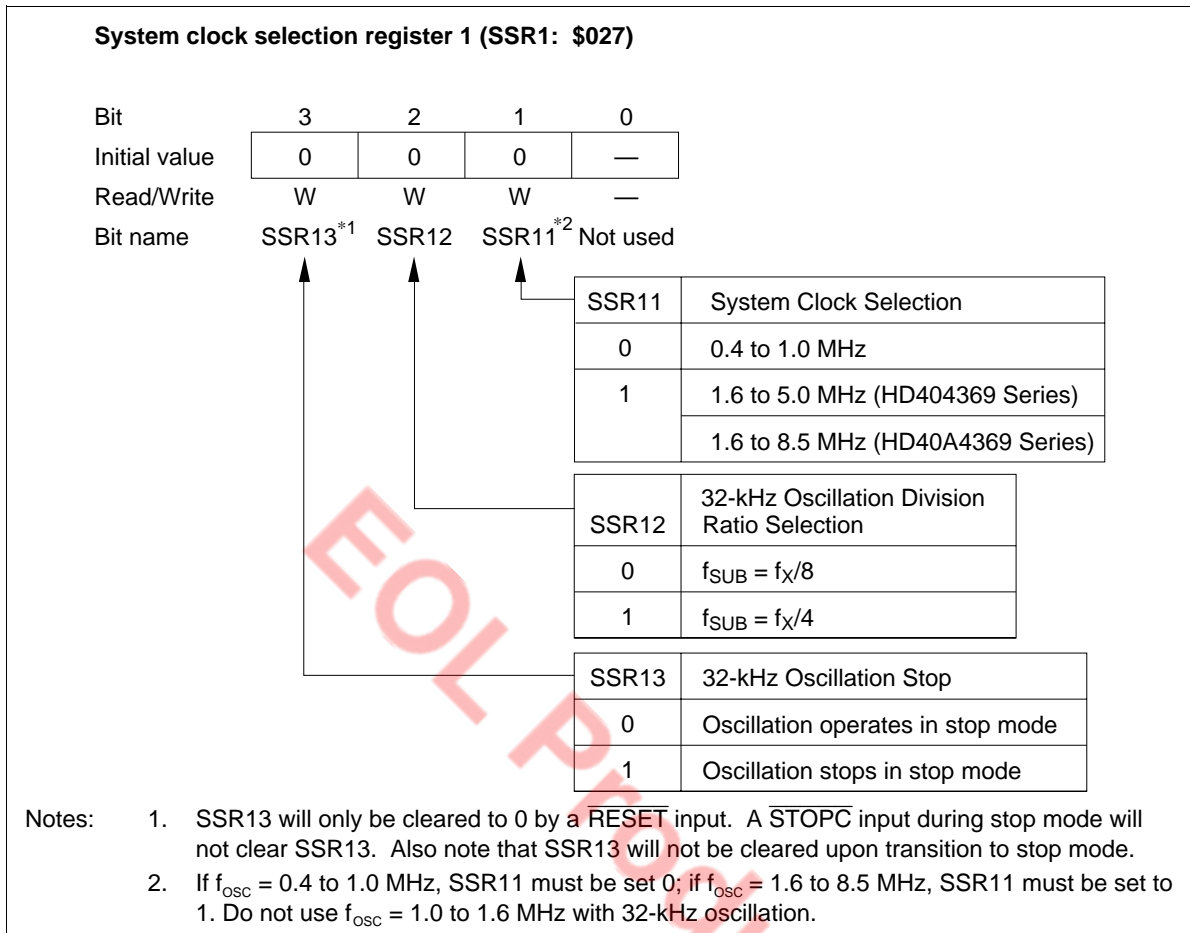
Figure 23 System Clock Selection Register 1 (SSR1)
