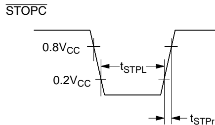
Figure 87 \overline{STOPC} Timing
