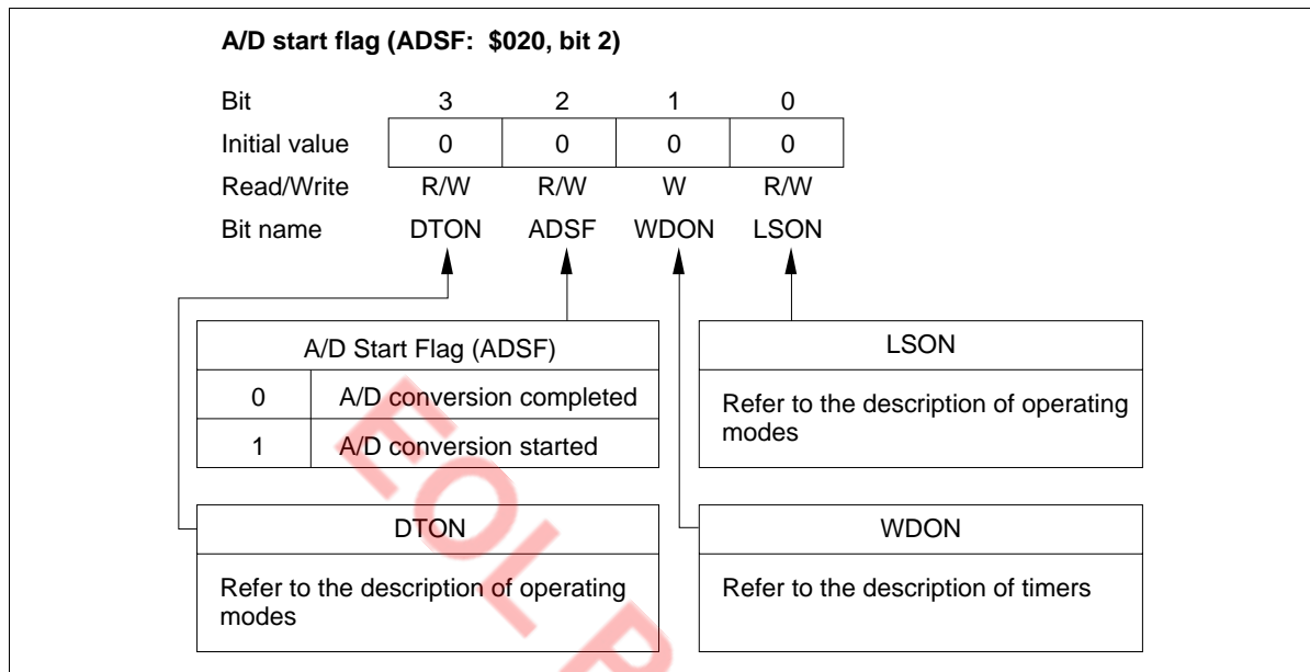
Figure 73 A/D Start Flag (ADSF)
