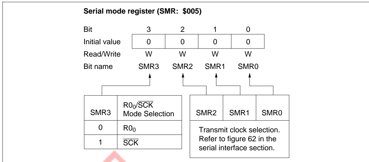
Figure 31 Serial Mode Register (SMR)
