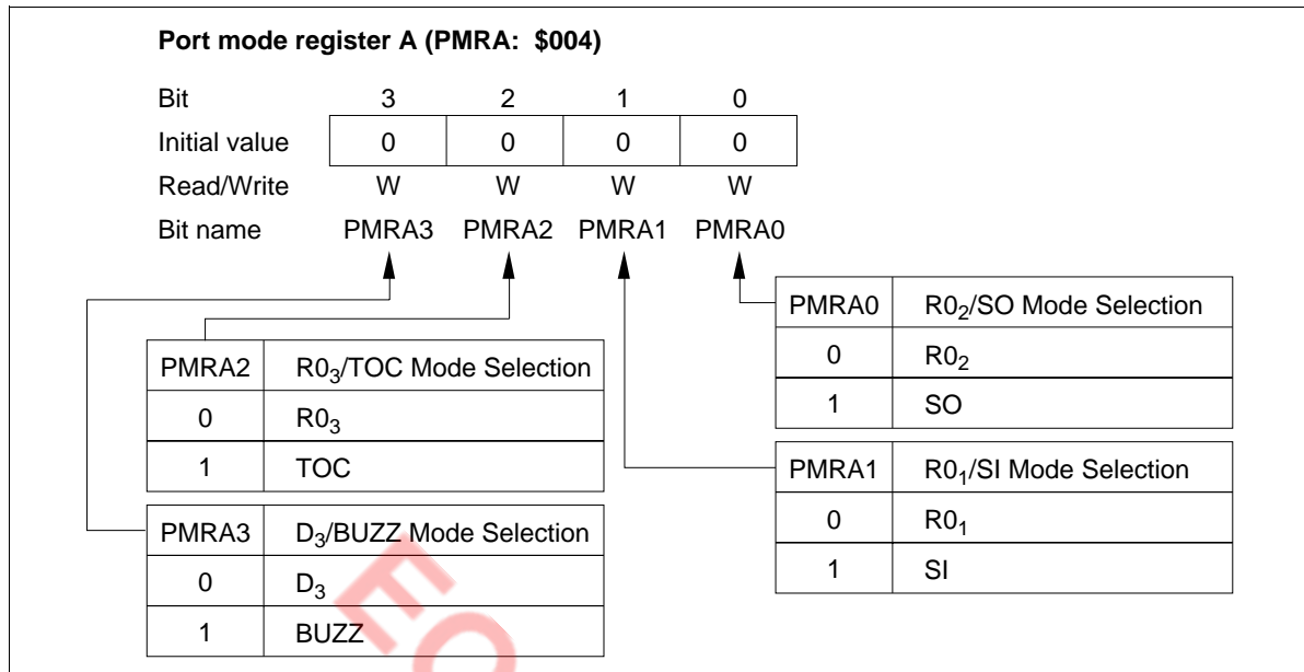
Figure 51 Port Mode Register A (PMRA)
