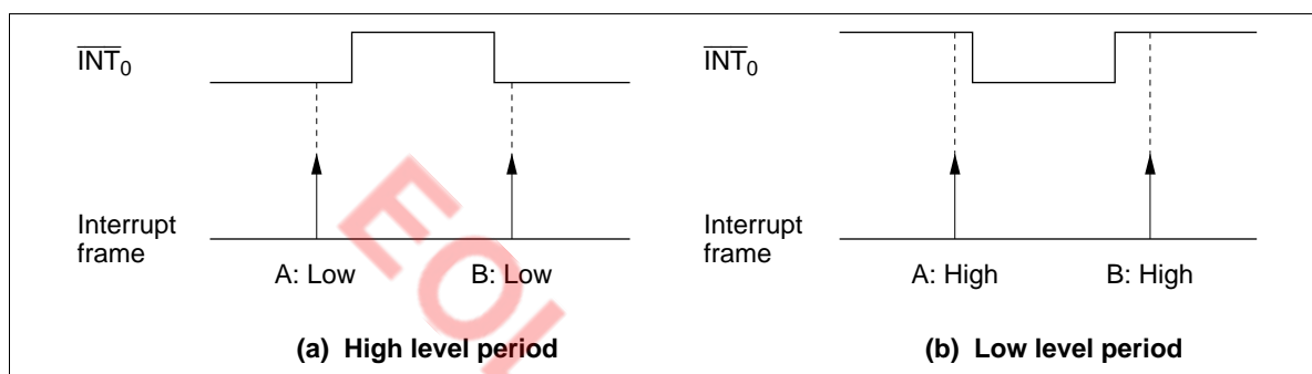
Figure 21 Sampling Example
