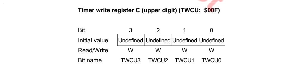
Figure 53 Timer Write Register C Upper Digit (TWCU)
