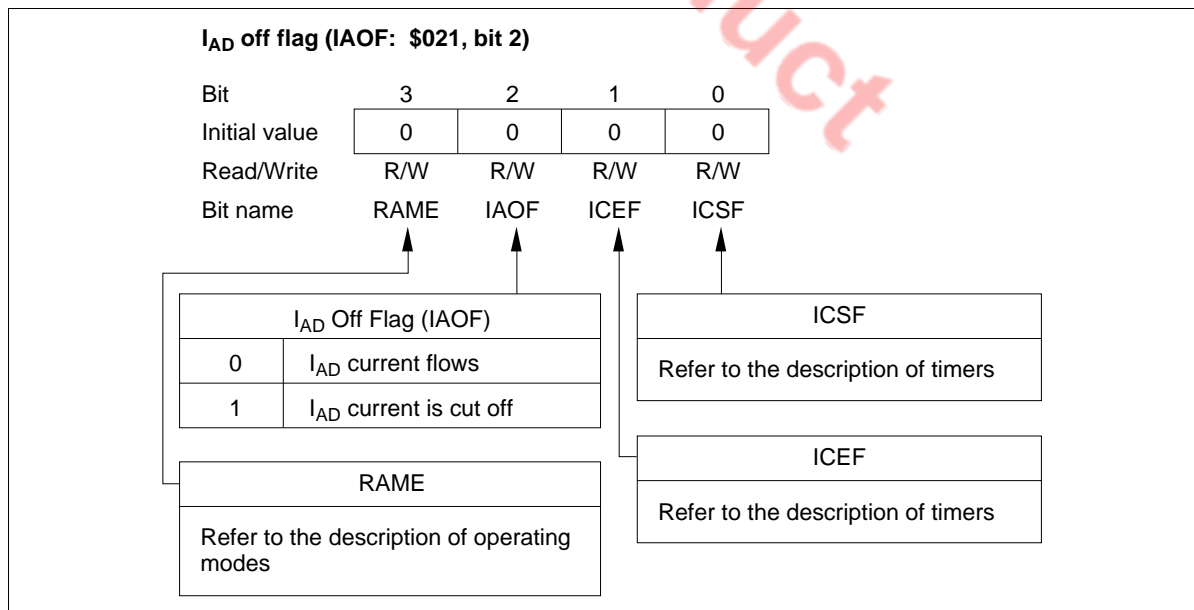
Figure 74 I AD Off Flag (IAOF)
