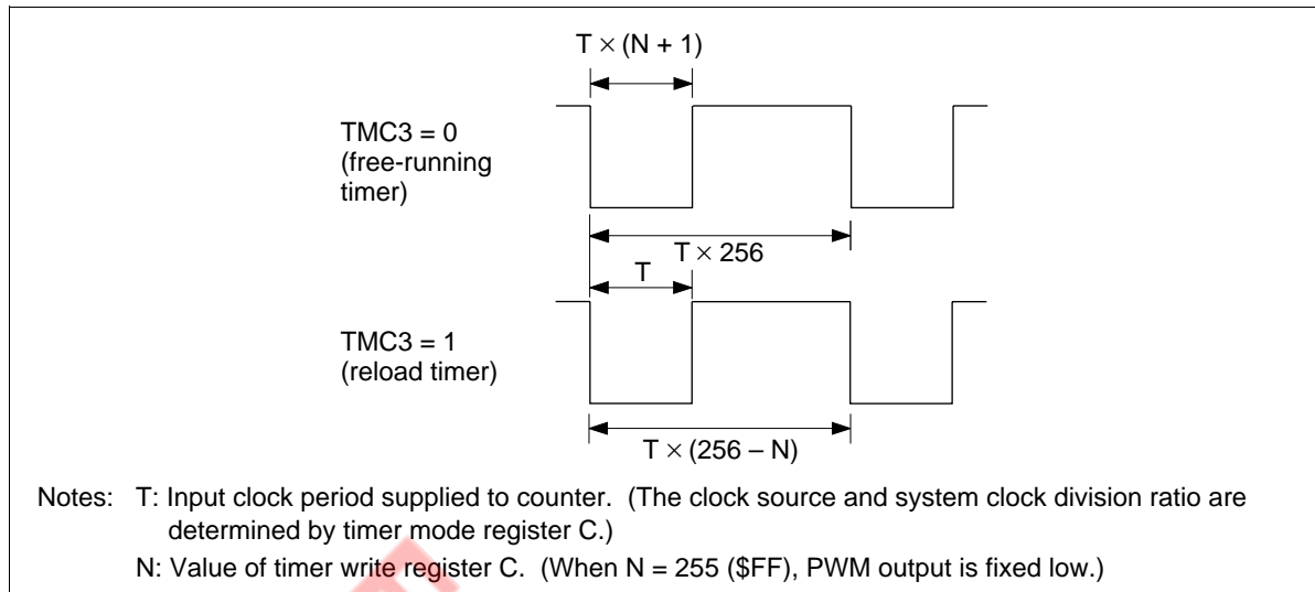
Figure 49 PWM Output Waveform
