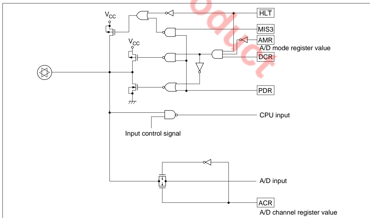
Figure 78 R Port/Analog Multiplexed Pin Circuit
