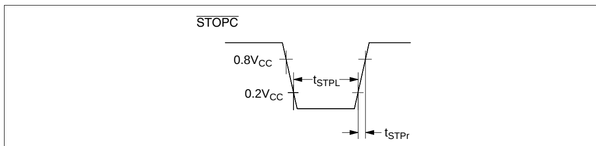
Figure 87 STOPC Timing
