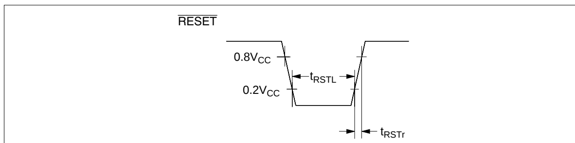
Figure 86 RESET Timing
