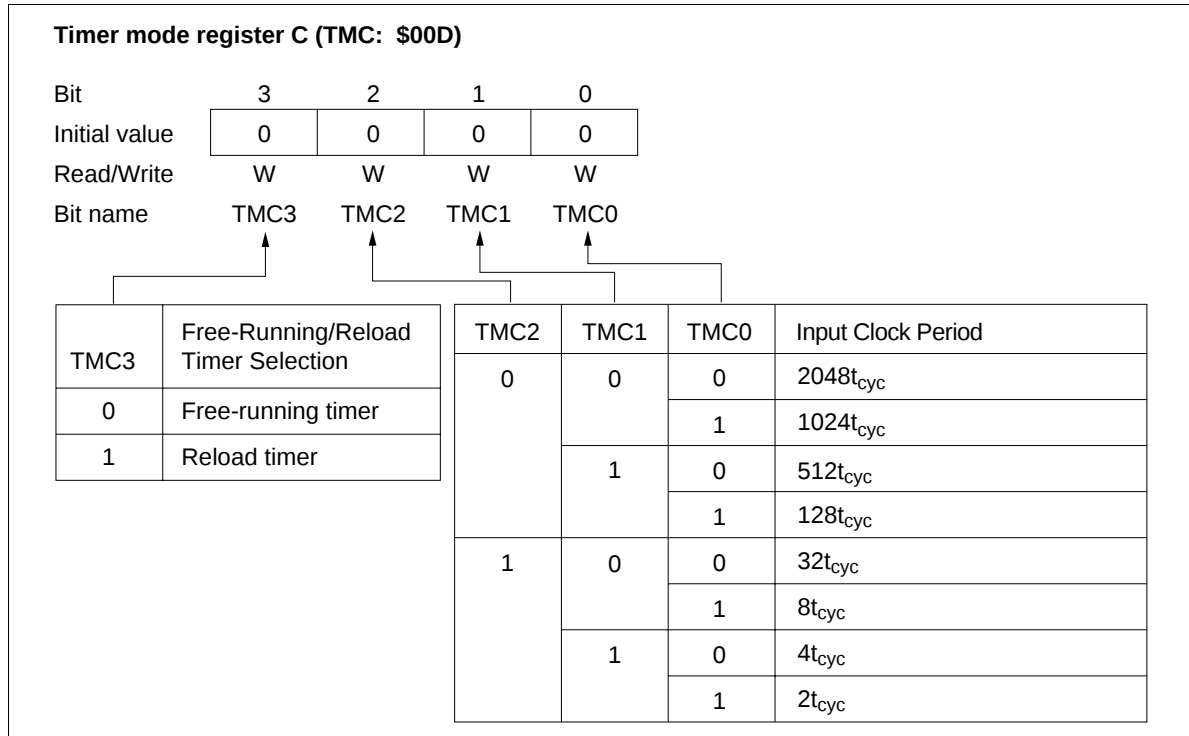
Figure 50 Timer Mode Register C (TMC)
