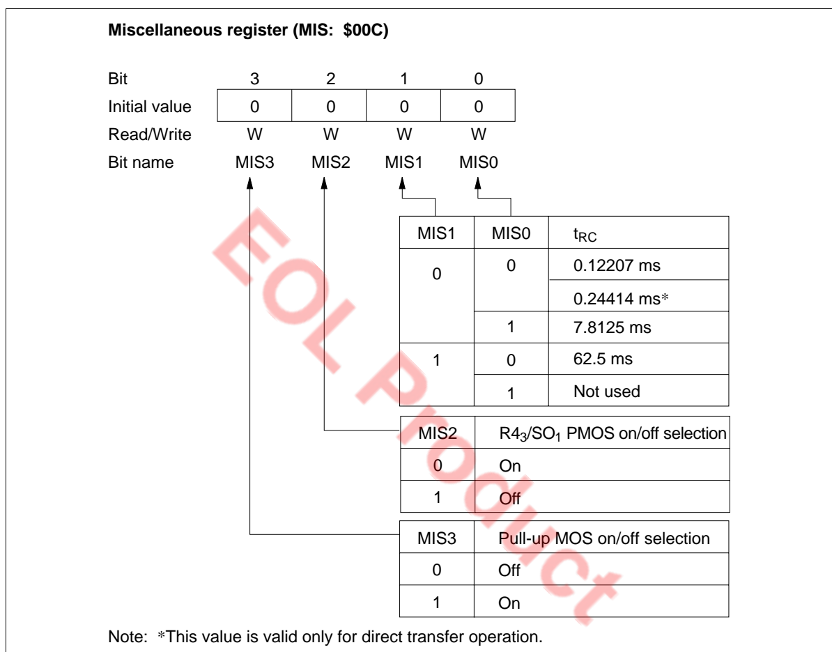
Figure 76 Miscellaneous Register (MIS)
