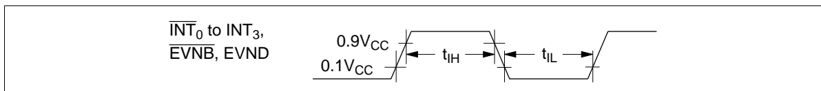
Figure 95 Interrupt Timing
