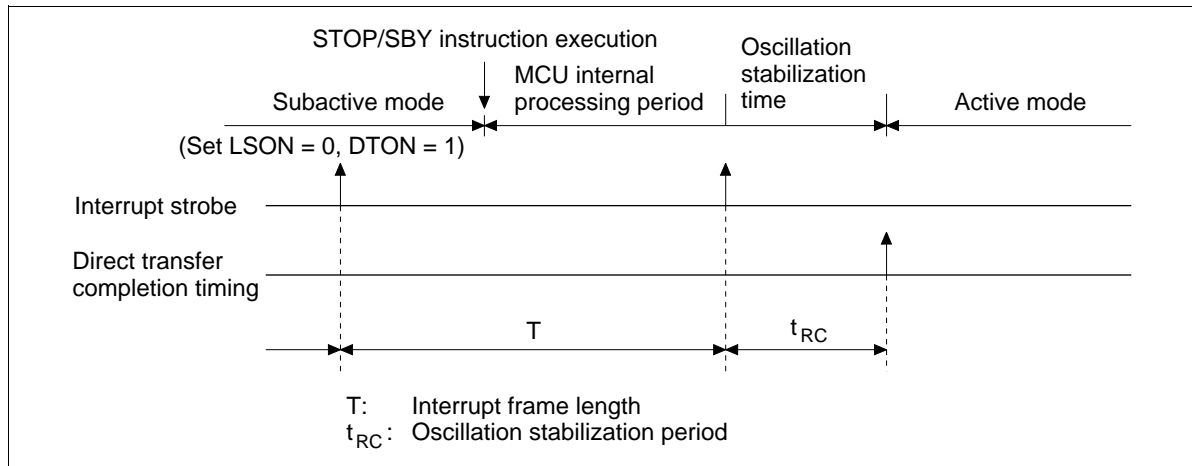
Figure 19 Direct Transition Timing
