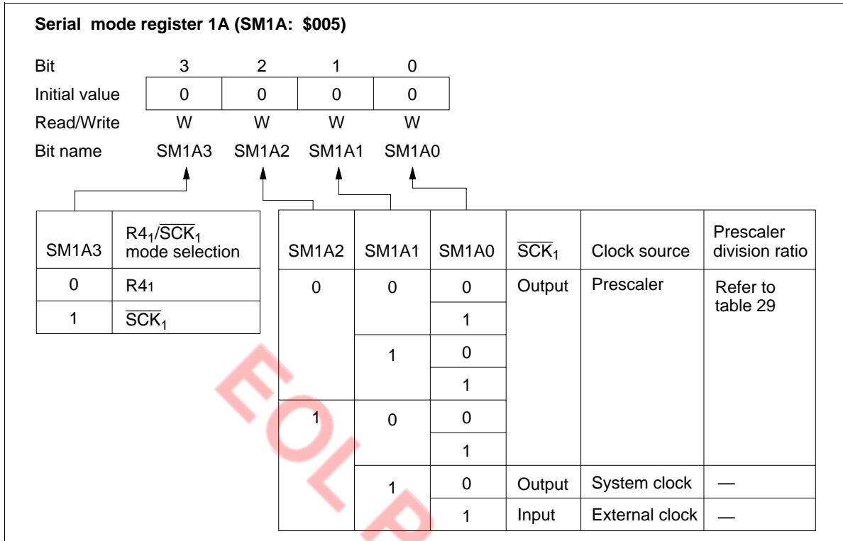
Figure 70 Serial Mode Register 1A (SM1A)
