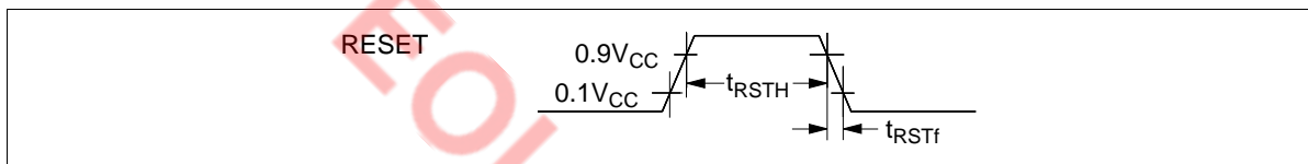
Figure 96 Reset Timing
