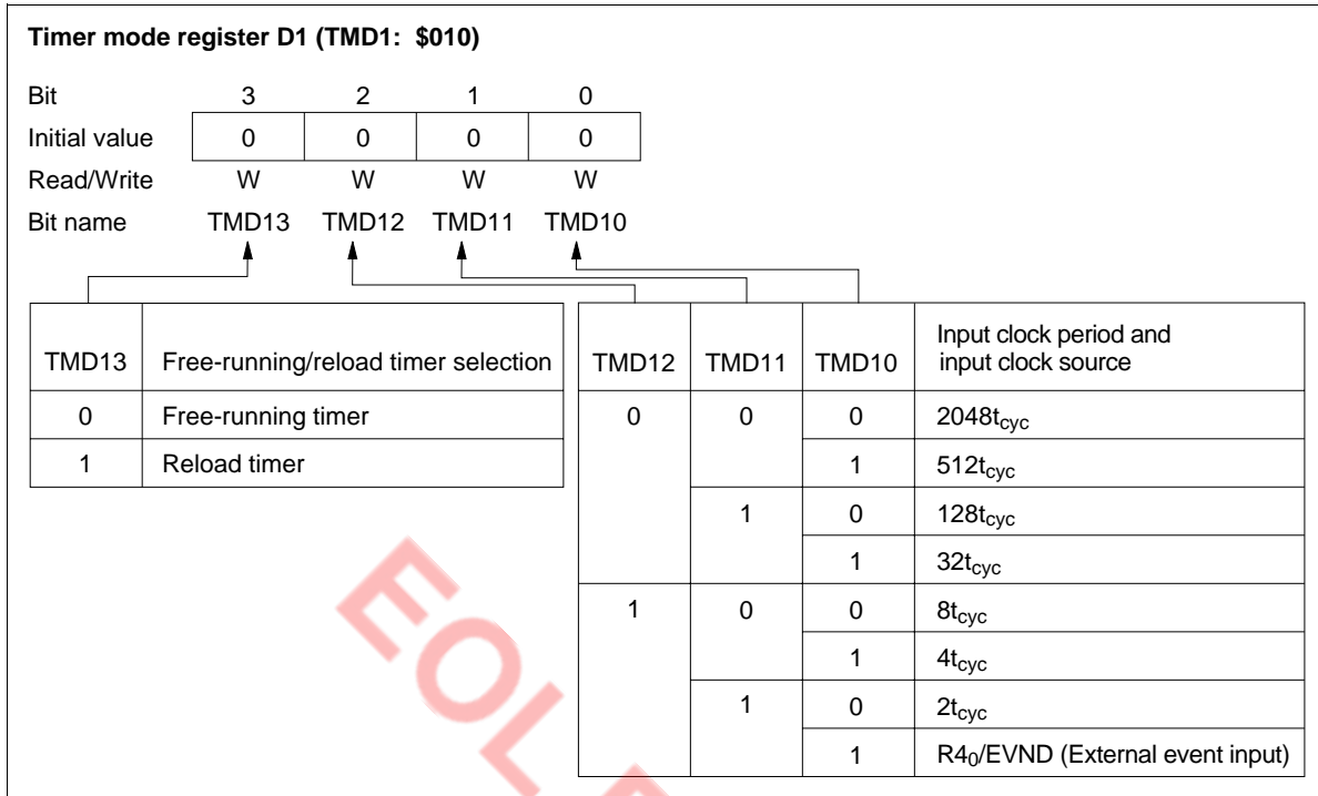
Figure 59 Timer Mode Register D1 (TMD1)
