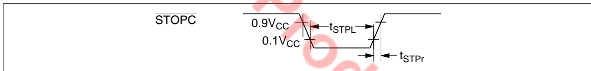
Figure 97 \overline{STOPC} Timing
