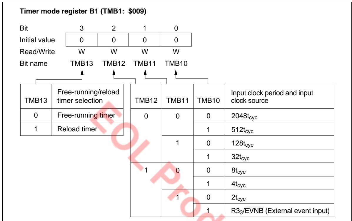
Figure 44 Timer Mode Register B1 (TMB1)
