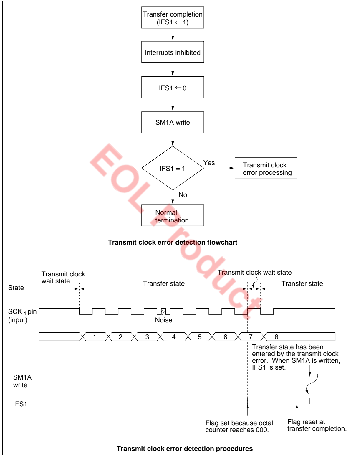
Figure 69 Transmit Clock Error Detection
