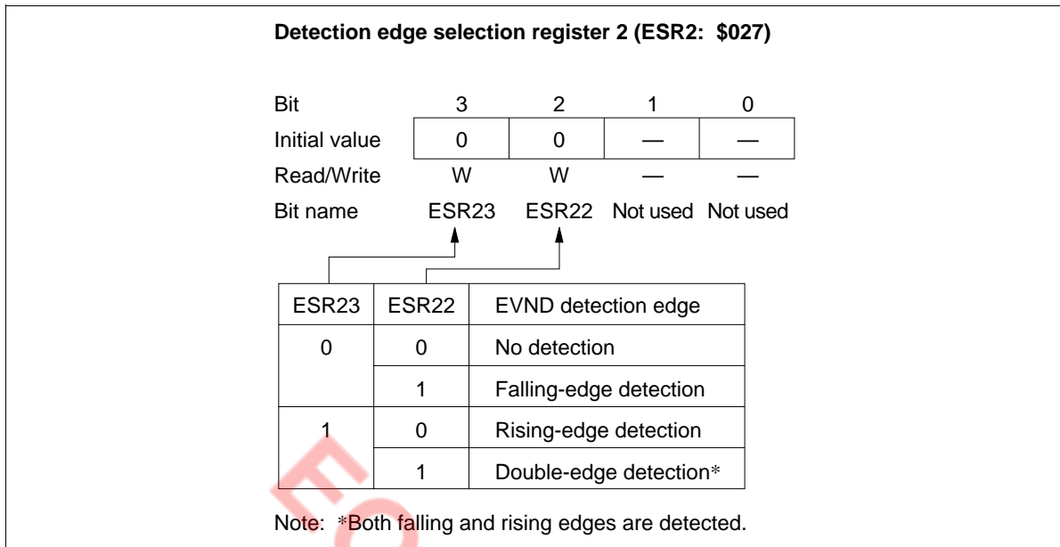
Figure 13 Detection Edge Selection Register 2 (ESR2)
