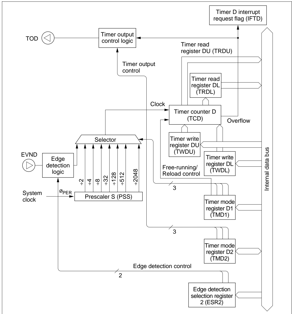
Figure 59(A) Block Diagram of Timer D (Free-Running/Reload Timer)
