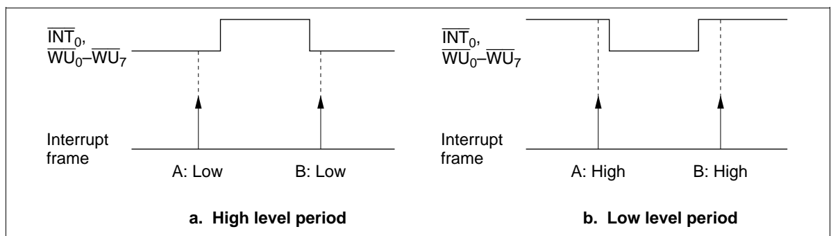
Figure 24 Sampling Example
