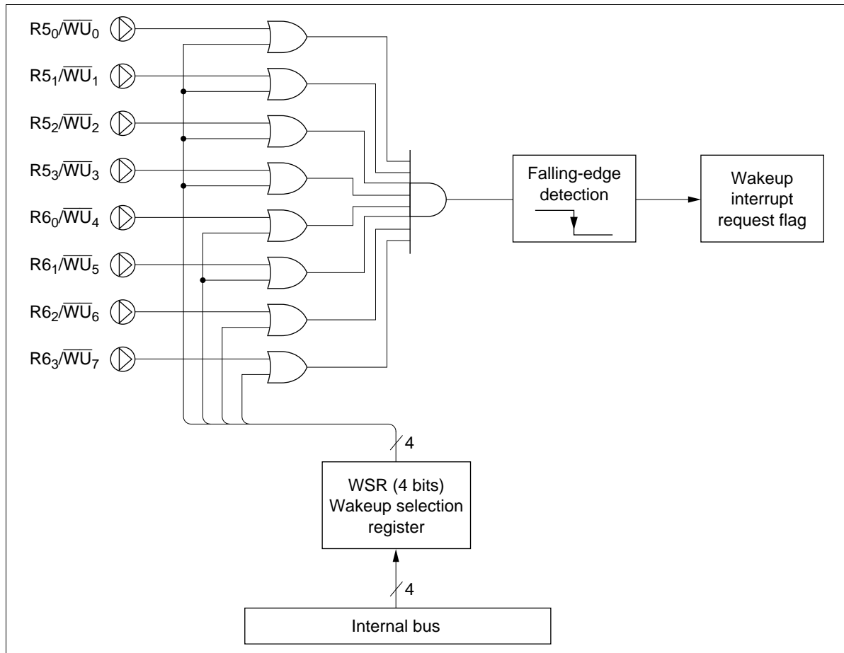
Figure 12 Wakeup Interrupt
