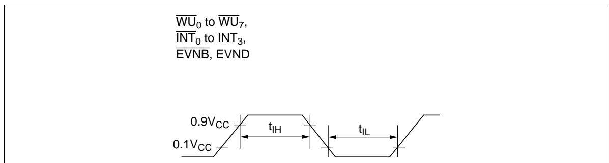
Figure 89 Interrupt Timing
