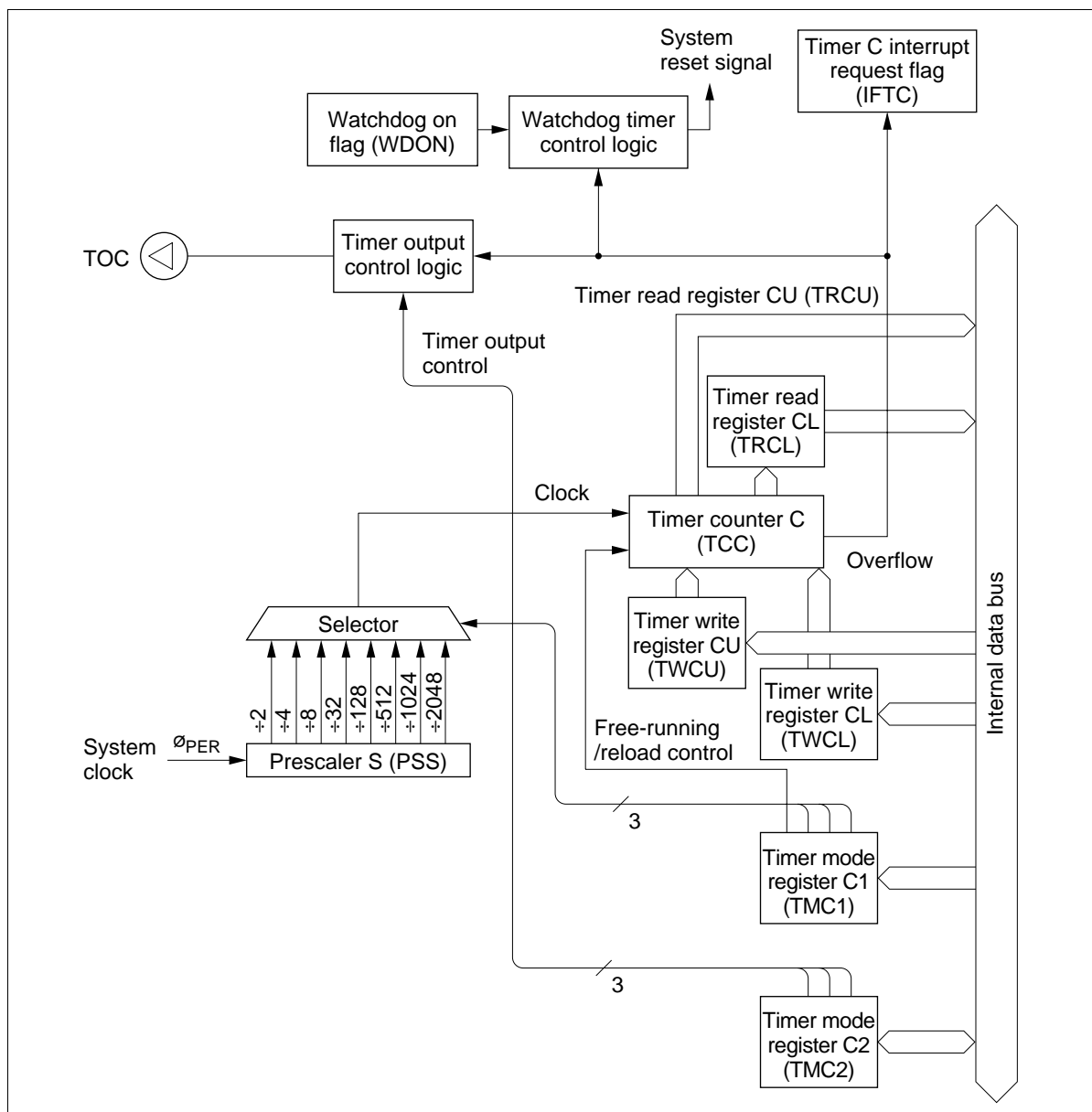
Figure 52 Block Diagram of Timer C
