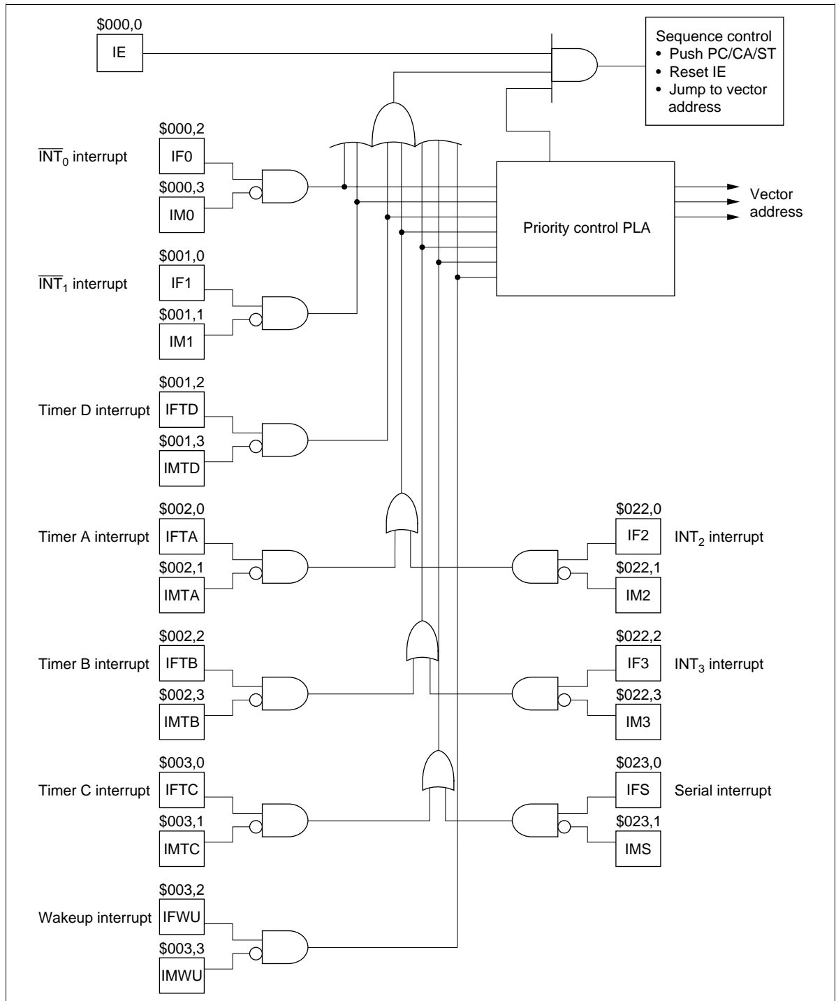
Figure 8 Interrupt Control Circuit
