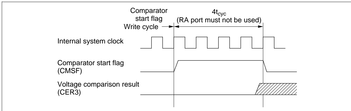
Figure 79 Comparator Operation Timing
