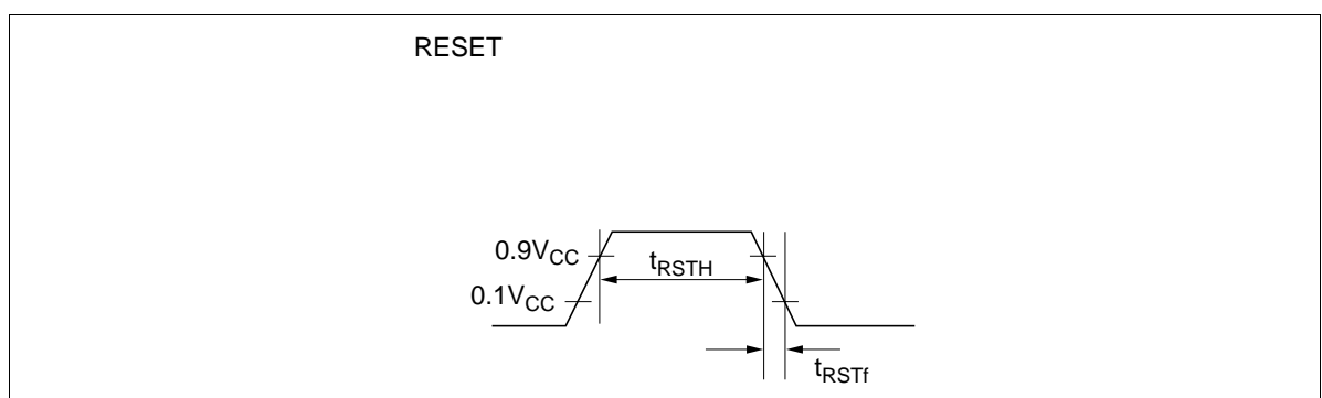
Figure 90 Reset Timing
