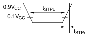
Figure 91 \overline{\text{STOPC}} Timing
