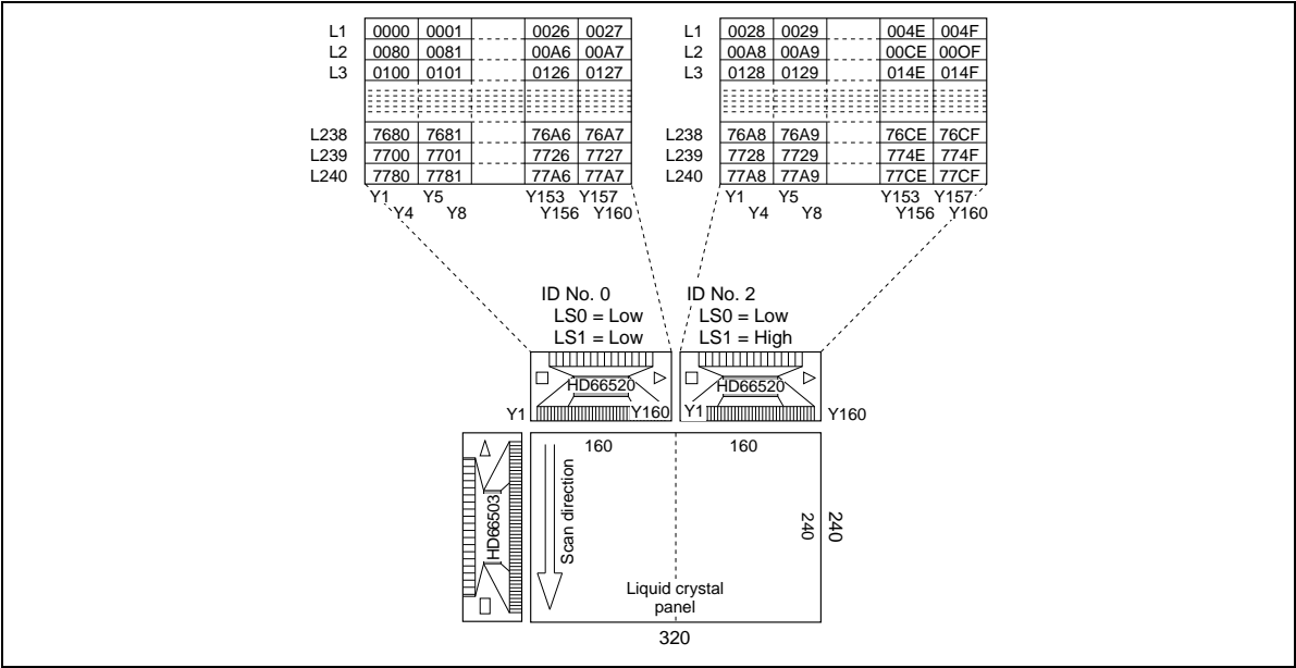
Figure 14 Quarter VGA Size (1)
