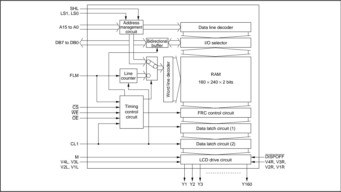
Figure 4 Block Diagram
