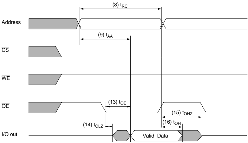
Read Cycle 1
