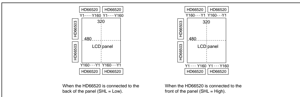
Figure 9 Address Assignment and SHL Pin Setting
