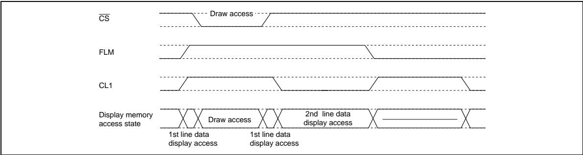
Figure 32 Draw Access (3)
