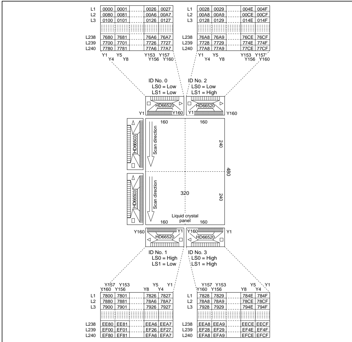
Figure 18 Half VGA Size (1)
