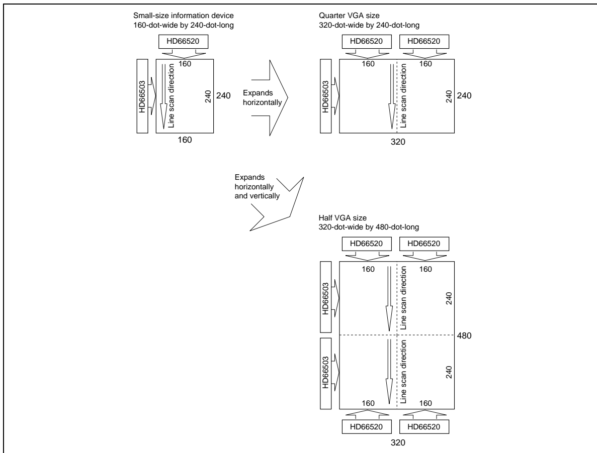
Figure 11 Application Examples
