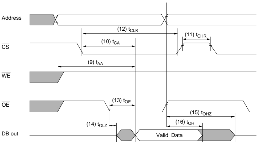
Read Cycle 2
