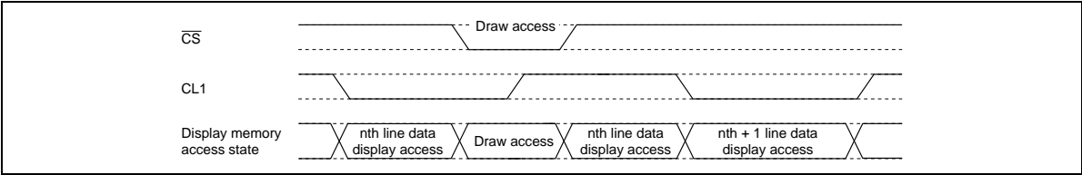
Figure 30 Draw Access (2)
