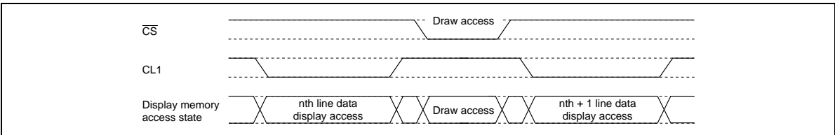
Figure 29 Draw Access (1)
