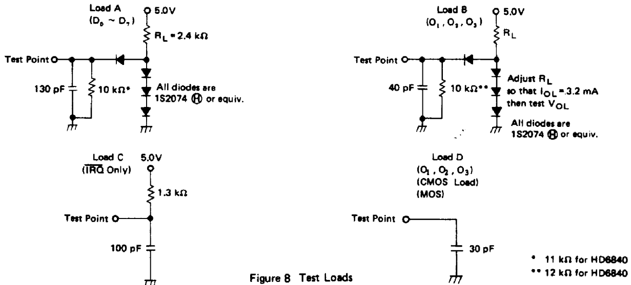
Figure 8 Test Loads
