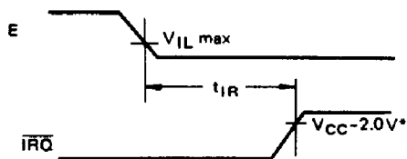
Figure 7 \overline{\text{IRQ}} Release Time
