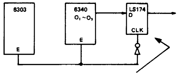
The latch added to prevent the noise (74LS174).
