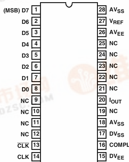
HI20203 (PDIP, SOIC) TOP VIEW
