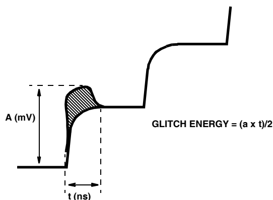
FIGURE 7. GLITCH ENERGY
