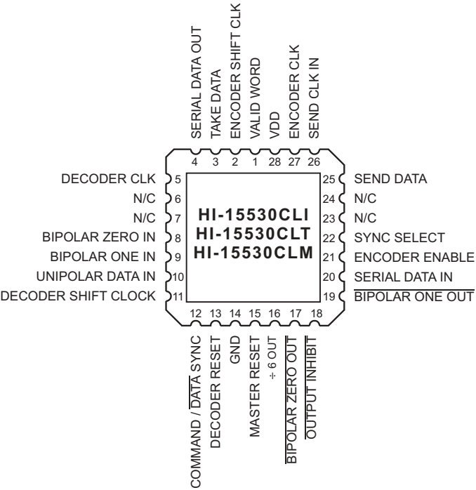
28 - Pin Ceramic LCC
