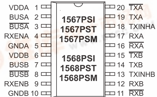
20 Pin Plastic ESD - WB package
