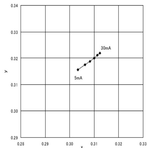
Forward Current vs. Chromaticity
