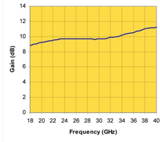
Linear Gain vs. Frequency
