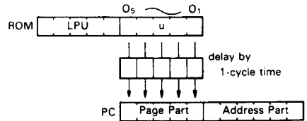
Figure 7 LPU Operation
