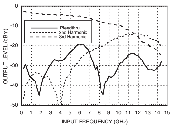
Output Harmonic
