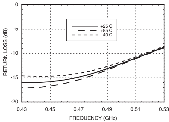
Input Return Loss vs. Temperature @ 470 MHz
