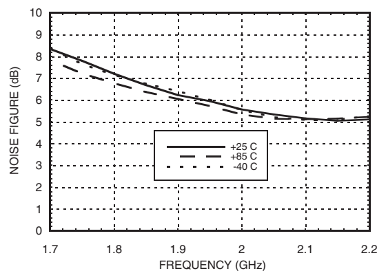
Noise Figure vs. Temperature @ 1960 MHz
