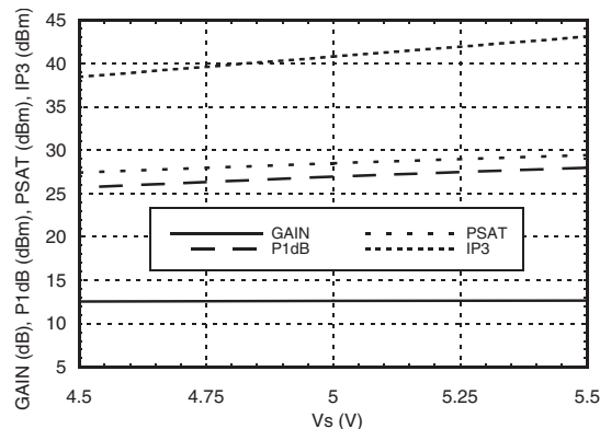
Gain, Power &amp; Output IP3 vs. Supply Voltage @ 1960 MHz
