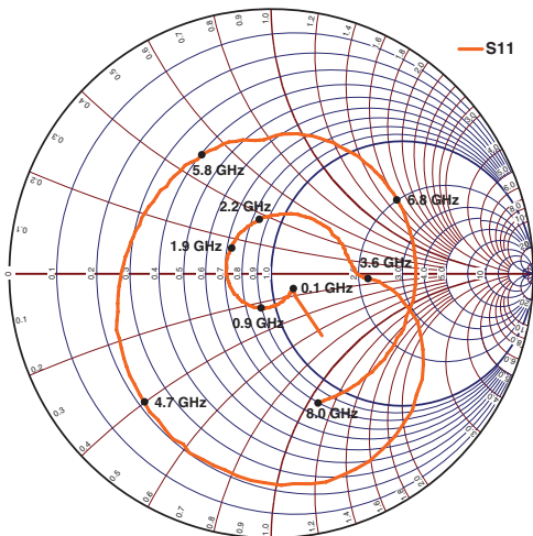
Input Impedance vs Frequency [3]
