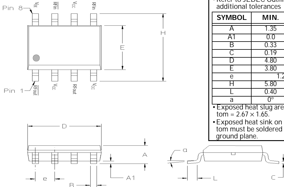
Figure 2. Package & Dimensions
