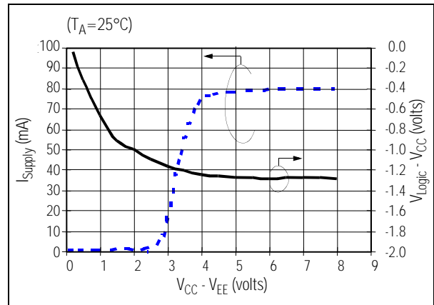
Figure 5. Typical Supply Current & V_{Loic} vs. Supply Voltage
