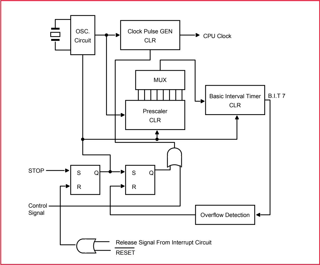
Figure 15-1 Block Diagram of Standby Circuit
