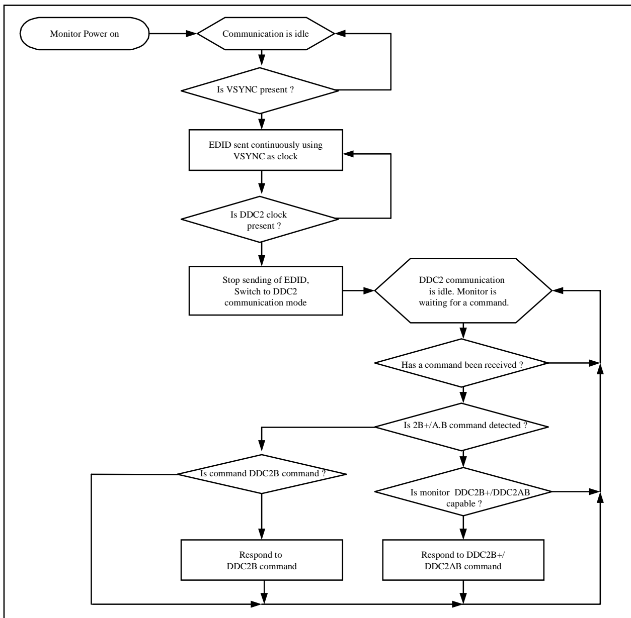
Figure 16-2 Host type detection
