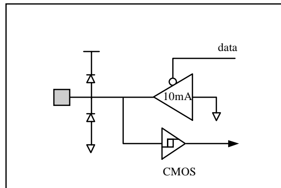
P0.6 - P0.7
