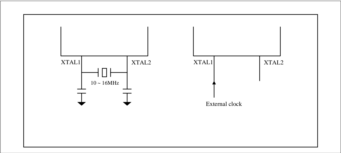
Figure 12-1 Oscillator configuration
