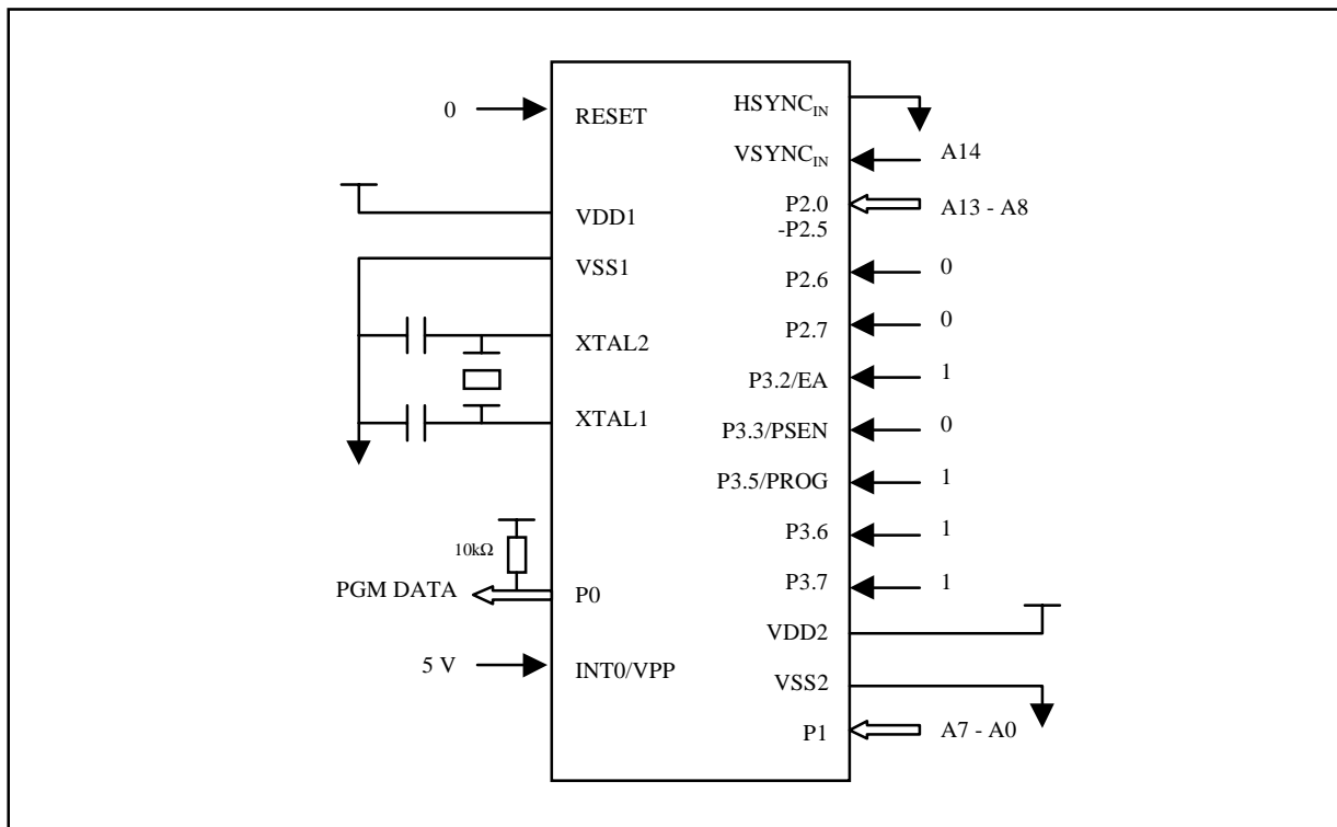
Figure 21-3 Verification Configuration
