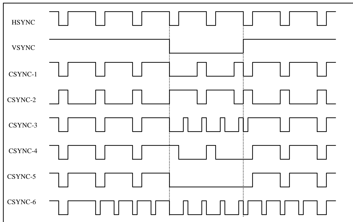
Figure 19-3 Non-standard composite sync signals
