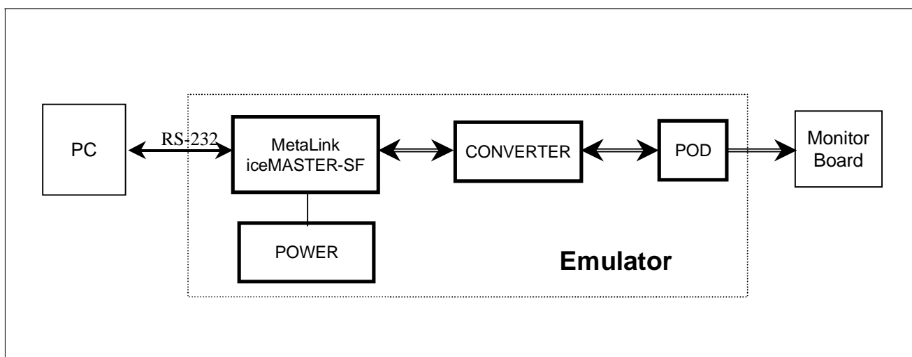
Figure 21-5 Development system Hardware Blockdiagram
