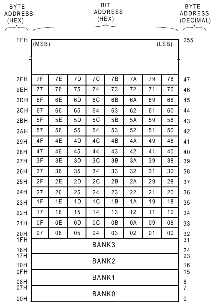
Figure 8-5 RAM ADDRESS
