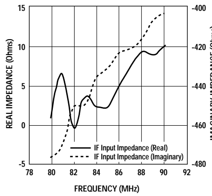
Figure 28. IF Input Impedance (differential) vs. Frequency. [1]
