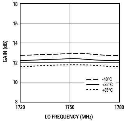
Figure 4. Gain vs. LO Frequency.
