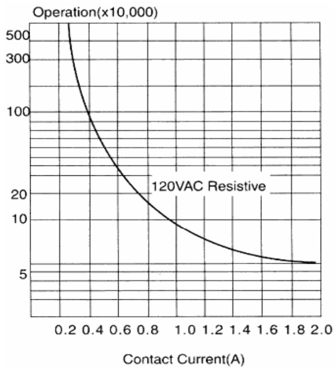
Life Curve
