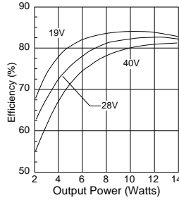
HR122-2815 Efficiency
