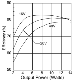
HR122-2812 Efficiency
