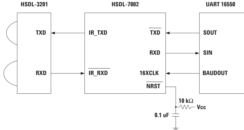
Figure 5. HSDL-7002 Connection between a standard 16550 UART and HSDL-3201
