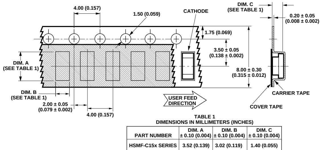
Figure 10. Tape Dimensions.
