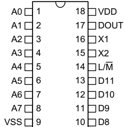
HT12A -18 DIP-A
