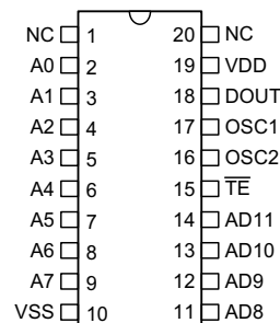
HT12E -20 SOP-A
