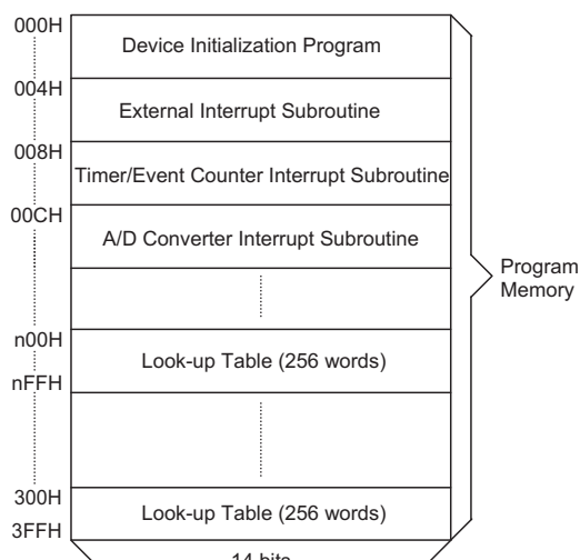
Program Memory
