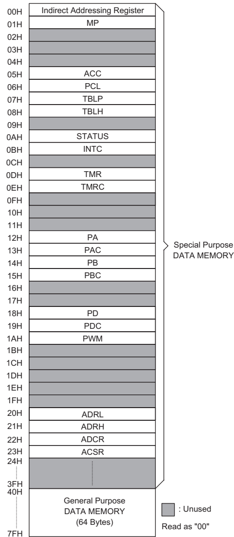
RAM Mapping
