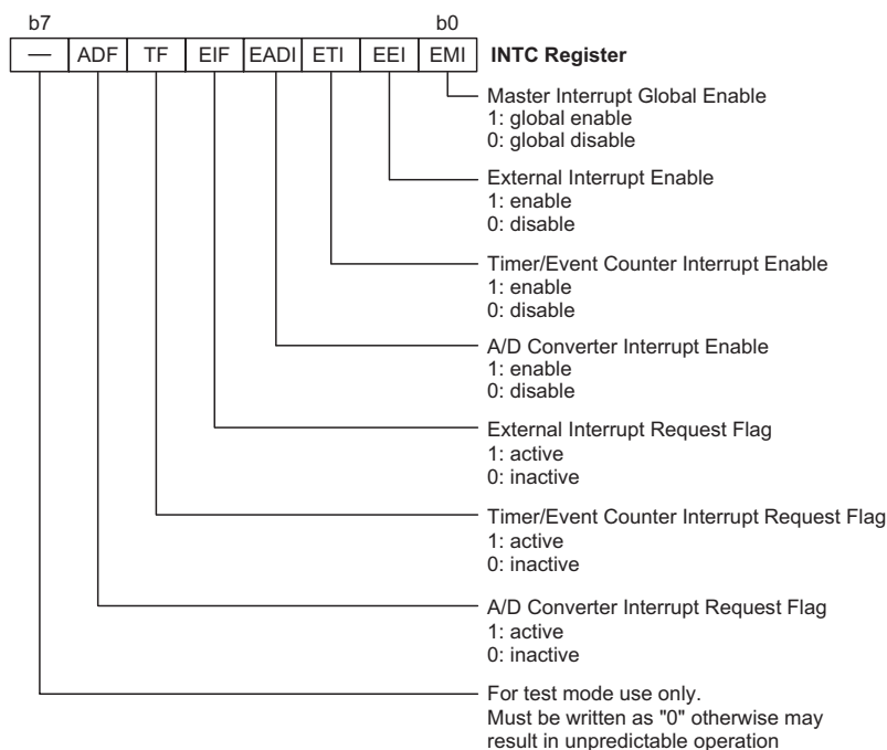
Interrupt Control Register
