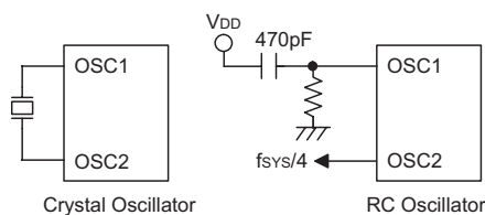
System Oscillator
