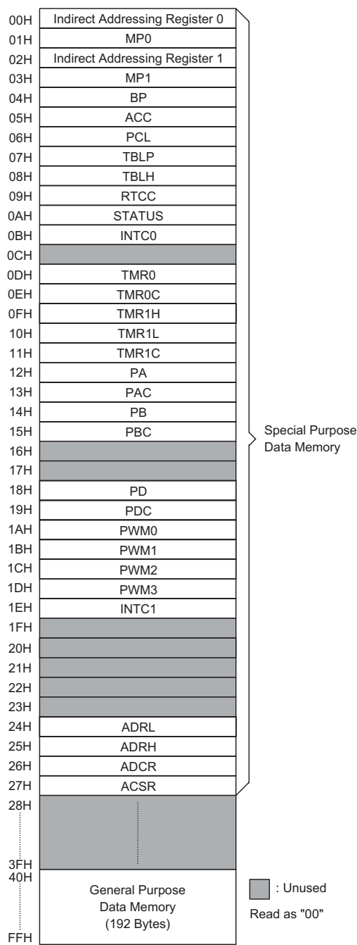
RAM Mapping
