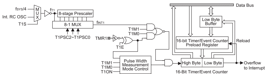
Timer/Event Counter 1
