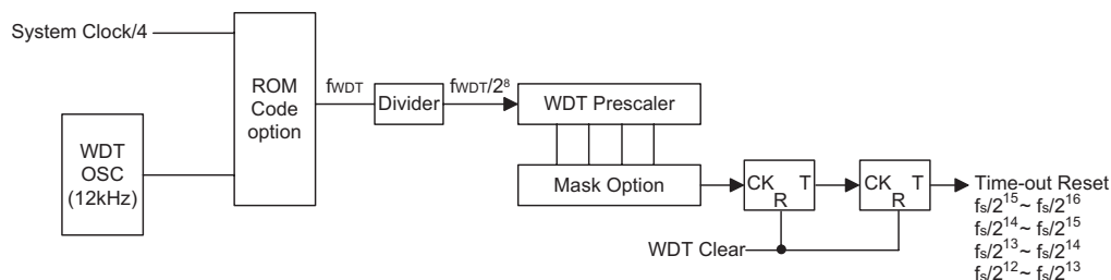
Watchdog Timer
