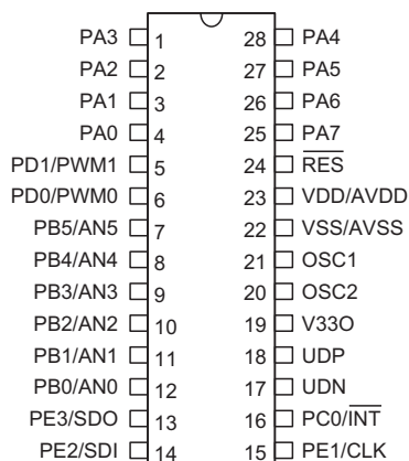
HT46RB50 – 28 SOP-A/SKDIP-A
